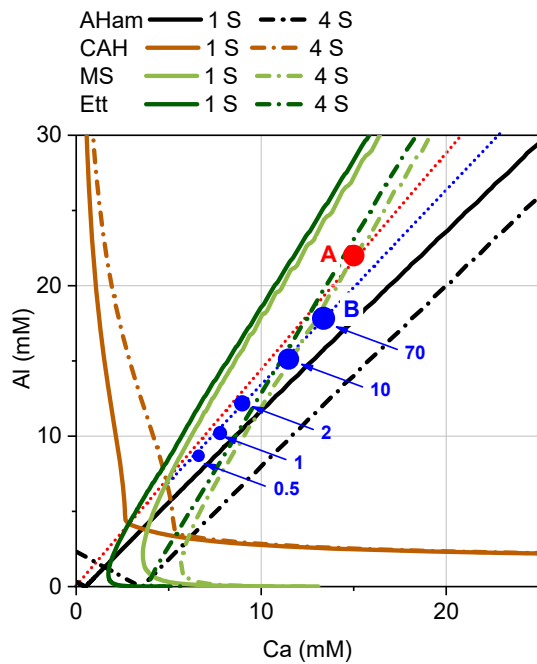
Figure 10 Intersections of surfaces of CAH - CAH 10 , MS
