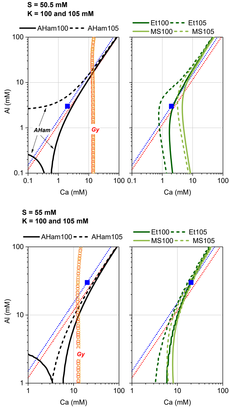
Figure 15 Intersections of solubility surfaces at S = 50.5 and 55 mM and two K concentrations equal to 100 and 105 mM. The straight blue dotted line shows the projection of theoretical dissolution line of ye'elimite on the Ca - Al plane. The square blue points depict the Ca and Al concentration corresponding to S = 0.5 at 1 mM from ye'elimite. The straight red dotted line shows the Ca/Al ratio corresponding to the dissolving C_{12}A_7 phase.
