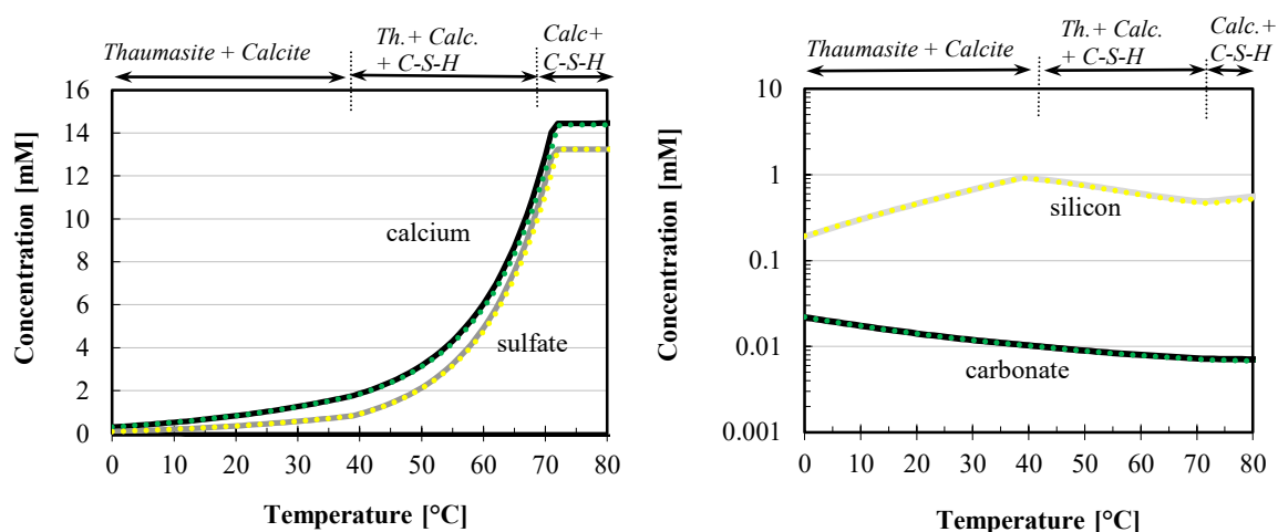
Figure B1. Calculated (curves) solubility data for thaumasite, based on the new thermodynamic data for thaumasite complemented with the CSHQ data from Cemdata18 [1, 7] in GEM format; Calculated (dotted lines) solubility data for thaumasite, based on data Cemdata18 [1, 7] in PHREEQC format.
