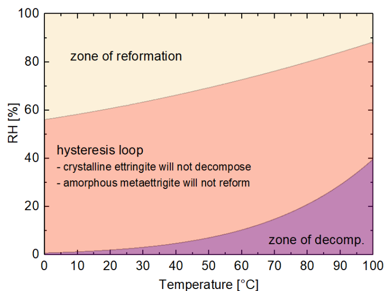
Figure 7: Stability of ettringite as a function of relative humidity and temperature.
