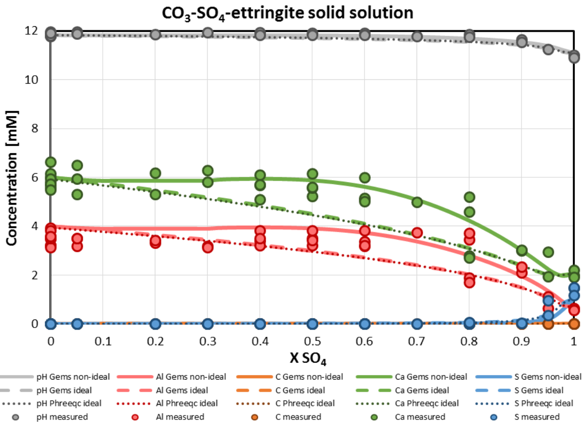
Figure B3. Calculated aqueous composition in equilibrium with \text{CO}_3\text{-SO}_4\text{-ettringite} solid solution as a function of \text{SO}_4 in the solid. Solid lines calculated using the Cemdata18 GEM format using non ideal solid solution; Dashed lines calculated using the Cemdata18 GEM format using ideal solid solution; Dotted lines calculated using the Cemdata18 PHREEQC format using ideal solid solution; Circles: experimental data [7, 129]
