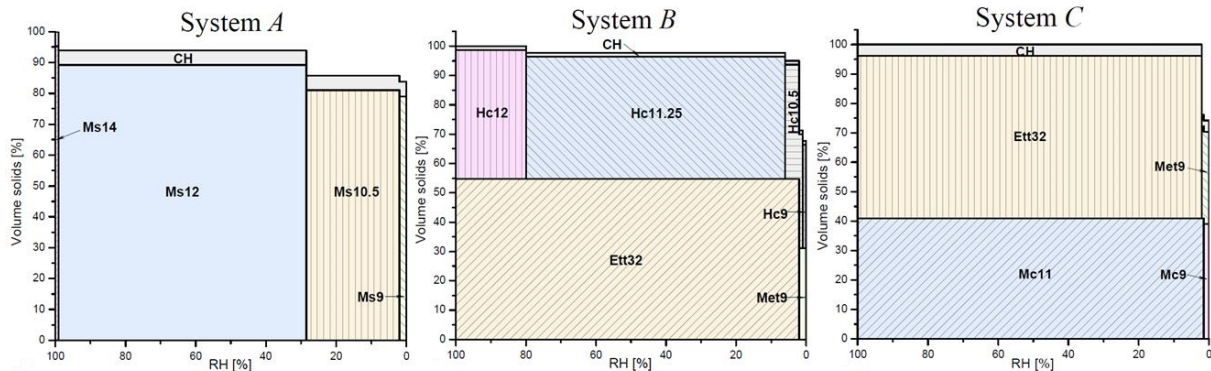
Figure 17: Calculated specific volume changes of a hydrated model mixture consisting of C_3A , portlandite and with fixed sulfate ratio ( SO_3/Al_2O_3=1 , molar bulk ratio) in dependence of changing calcite content at 25°C, as shown in Figure 16 for the Systems A, B and C.
