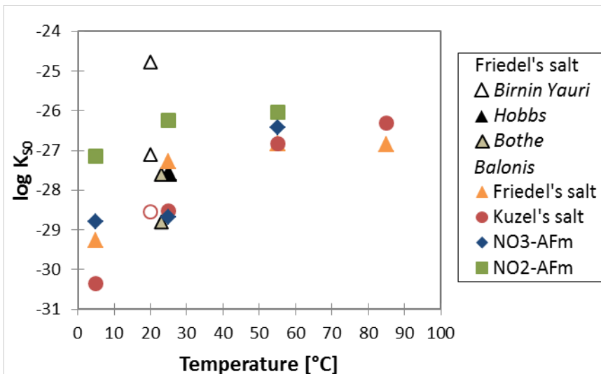
Figure 4: Solubility products of Friedel's salt, Kuzel's salt, NO 3 -AFm and NO 2 -AFm (referring to reactions using Ca 2+ , Cl - , SO 4 2- , NO 3 - , NO 2 - , OH - and H 2 O as indicated in Table 2) as a function of temperature. Data for Friedel's salt from [27, 58-60, 62], data for other AFm are from Balonis and co-workers [27, 34-36].
