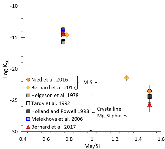
855 856 Figure 11: Evolution of the solubility product ( K_{s0} ) of magnesium silicate hydrates at room temperature 857 as a function of the total Mg/Si; referring to reactions using \text{Mg}^{2+} , \text{SiO}_2 and \text{H}_2\text{O} as indicated in Table 858 2. Adapted from [118].
